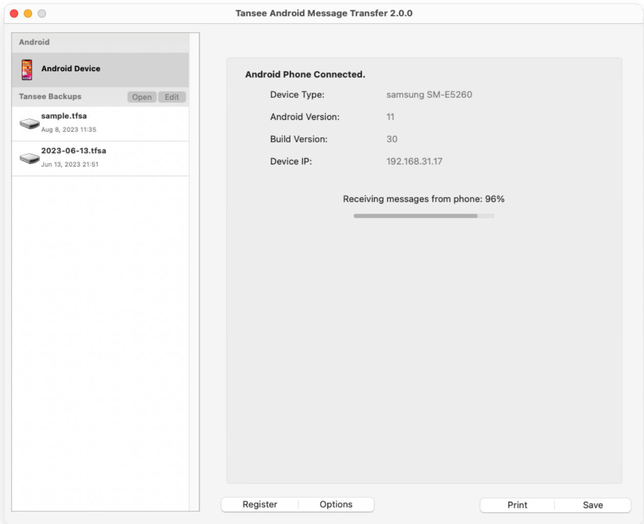
Loading Messages
